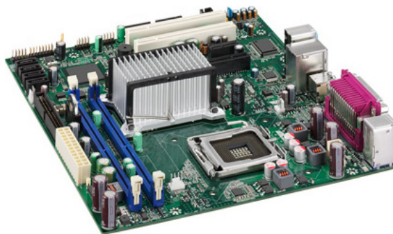
Figure 1. - Intel DG41TY motherboard
