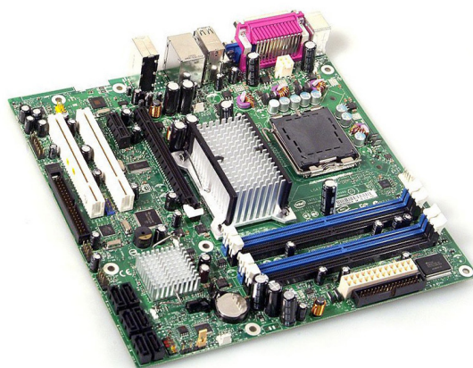
Figure 1. - Intel DQ965GF motherboard
