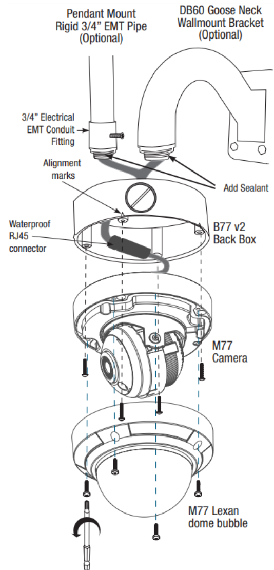
B77 v2, Back box for M77.
